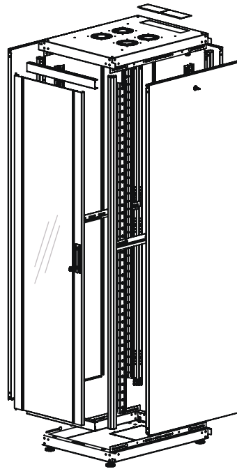
EXPLODED VIEW
