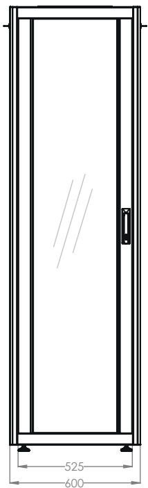
FRONT VIEW
